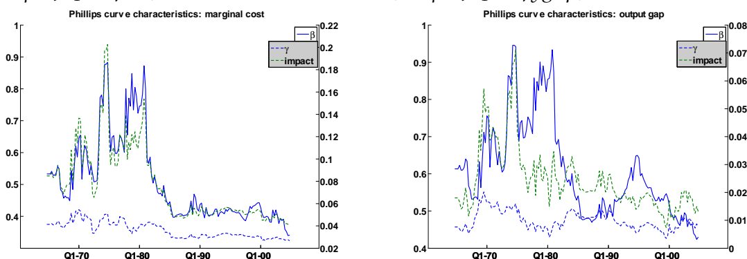
Figure 12. Phillips curve parameters implied by the learning model.
