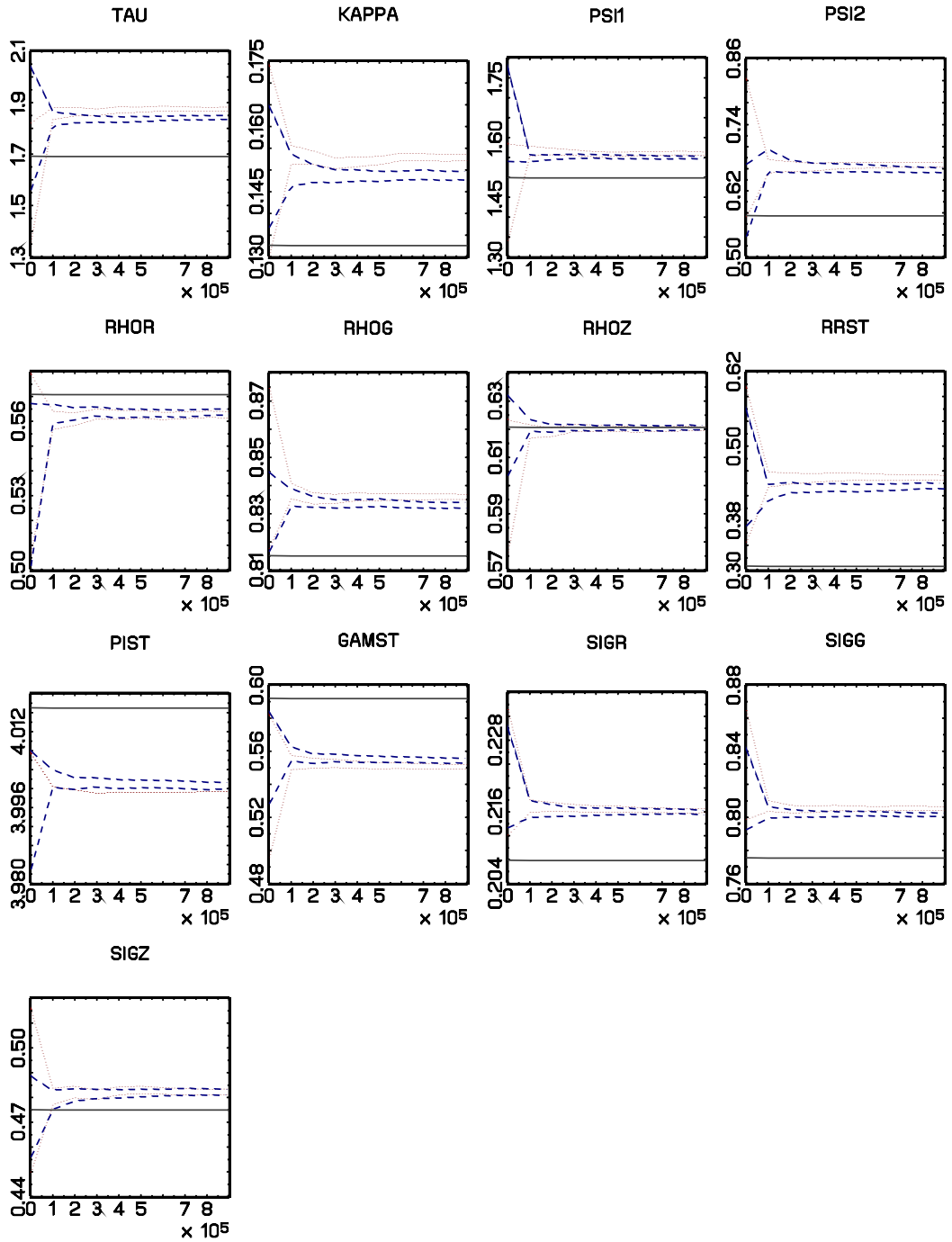
Figure 4: METROPOLIS ALGORITHM VERSUS IMPORTANCE SAMPLING
