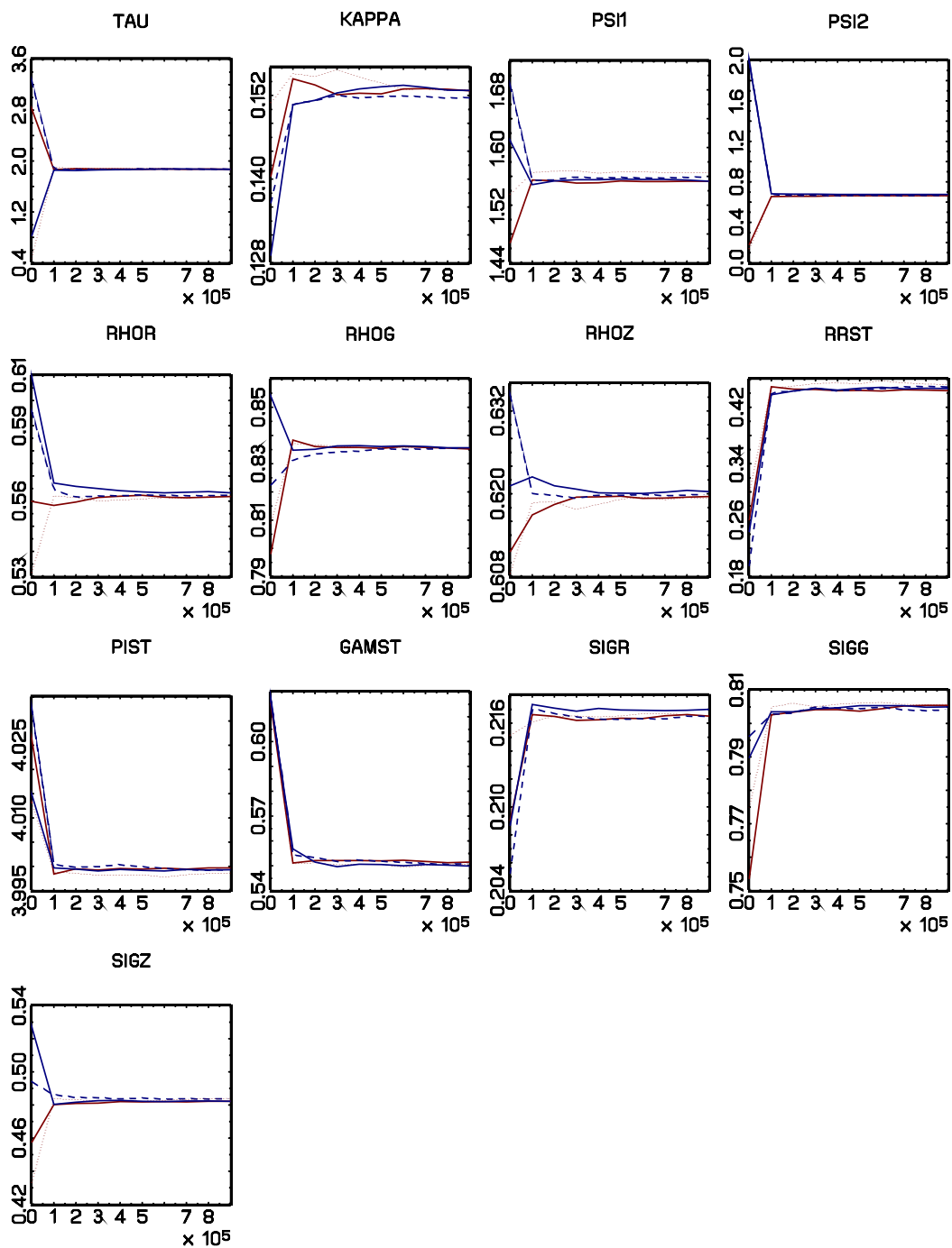
Figure 3: RECURSIVE MEANS FROM MULTIPLE CHAINS
