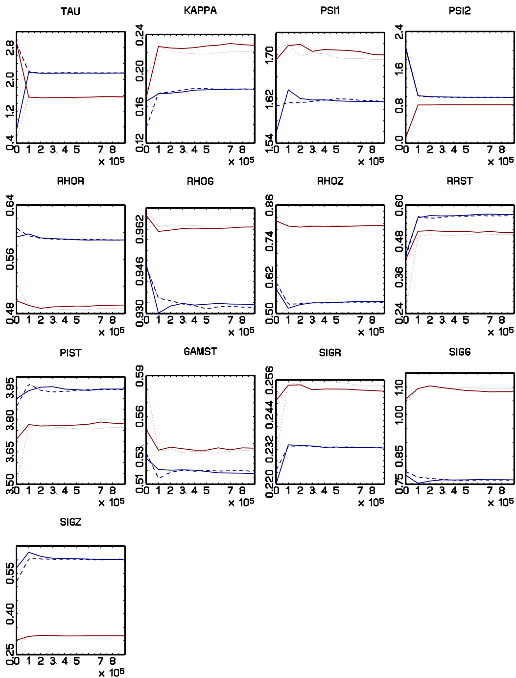
Figure 6: RECURSIVE MEANS FROM MULTIPLE CHAINS
