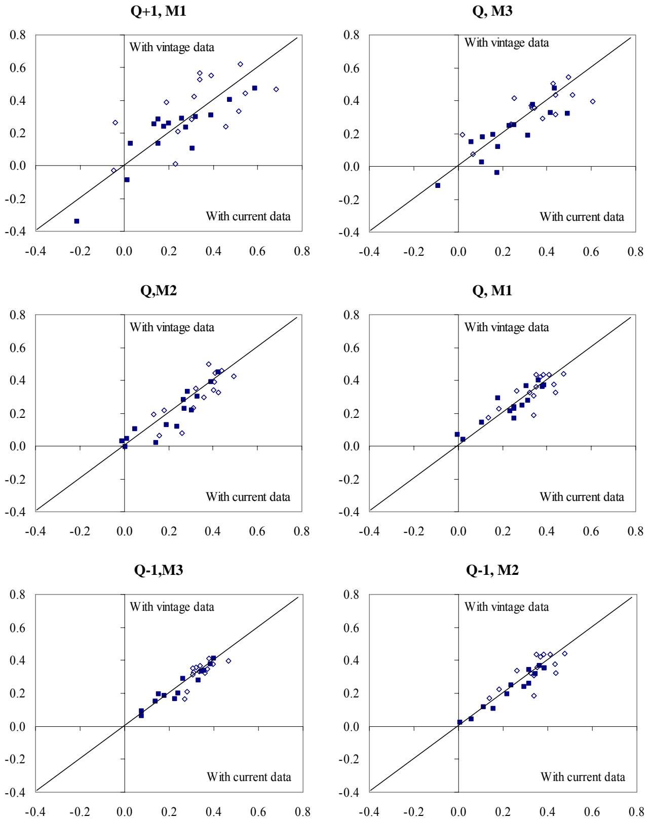
Figure 5 – Forecasts from equations (1) and (2) based on current estimates and real-time data Quarter-on-quarter growth rates
