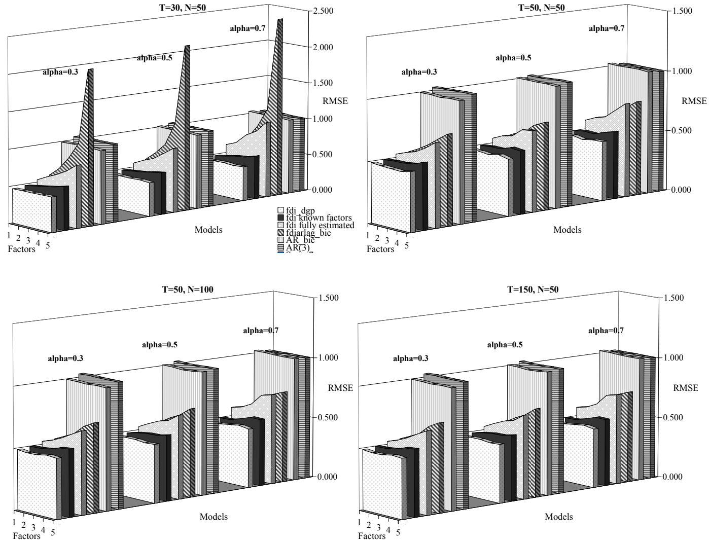
Figure 3: Time variation in factor loadings, h = 1
