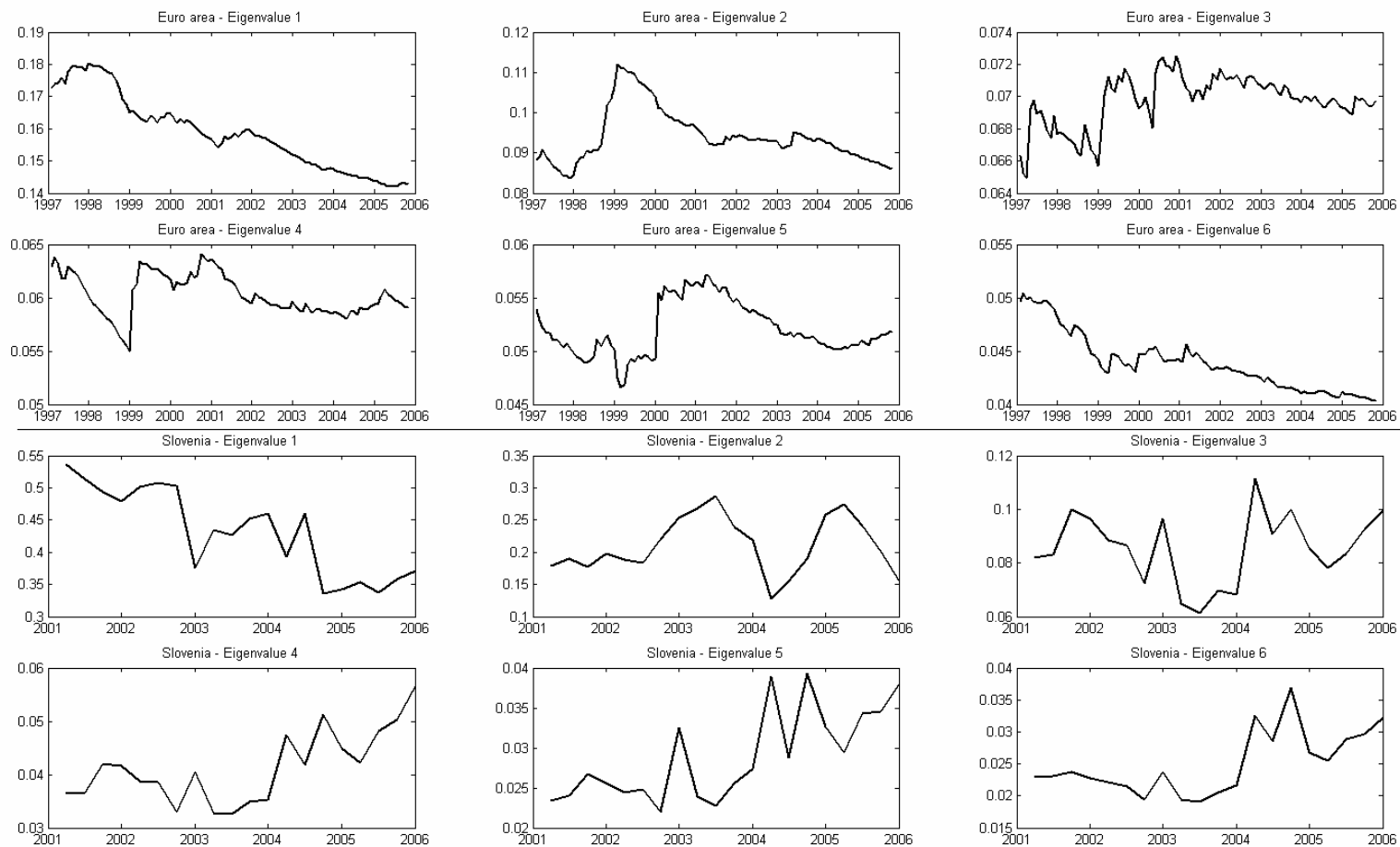
Figure 10: Recursive normalized eigenvalues
