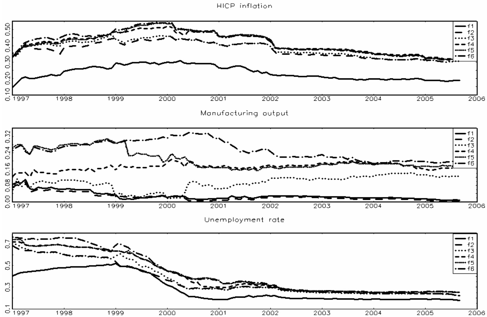
Figure 6: Recursive adjusted R^2 , h = 1 , Euro area
