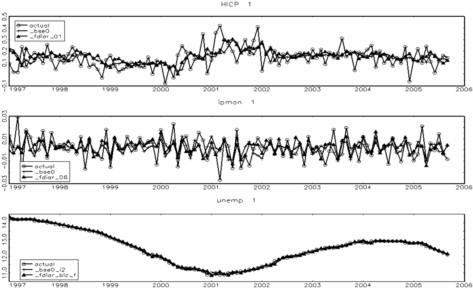
Figure 12: Forecasting macroeconomic variables for the Euro area, sample 1991 – 2005
