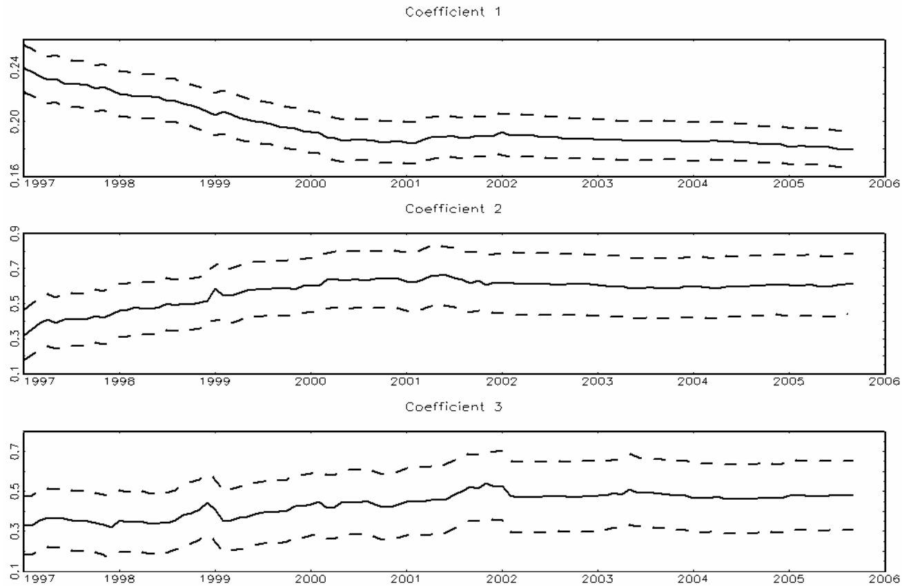
Figure 7: Euro-area inflation: Recursive Coefficients from fac_fdiarlag_bic Model
