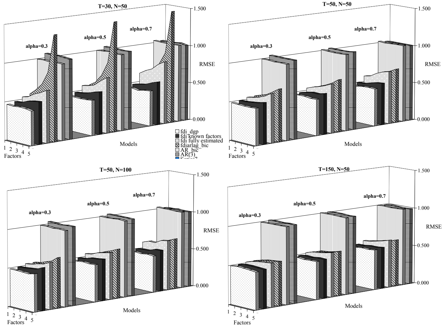
Figure 1: Basic DGP, h = 1
