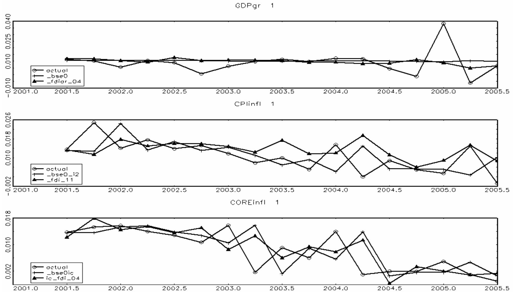
Figure 13: Forecasting macroeconomic variables for Slovenia
