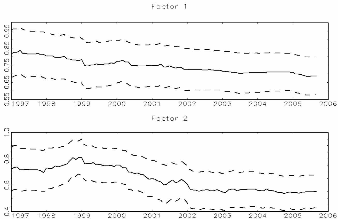
Figure 11: Recursive persistence of factors, Euro area, sample 1991 – 2005
