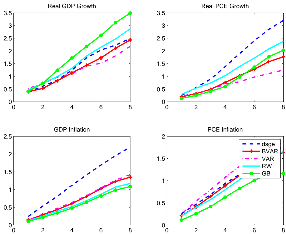
Figure 1: MAEs of Different Models and Greenbook (August 1996 - May 2000)
