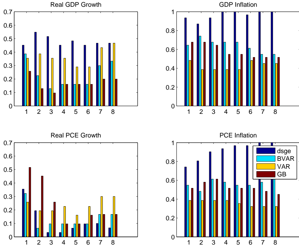
Figure 3: Forecast Bias of Different Models and Greenbook (August 1996 - May 2000) (Figure displays the fraction of periods for which the model's forecast is greater than zero)
