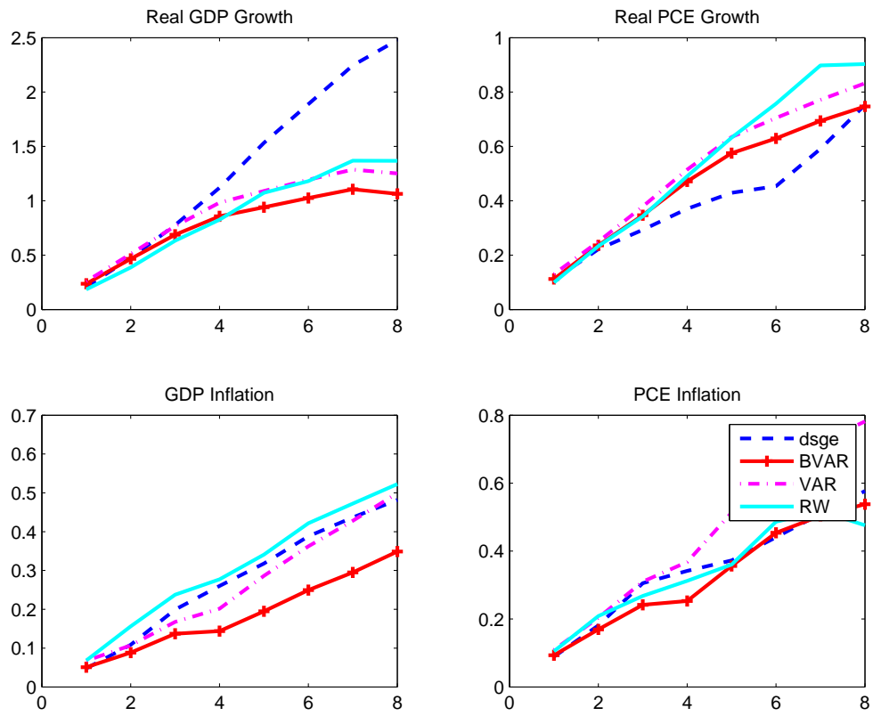
Figure 2: MAEs of Different Models and Greenbook (June 2000 - Jun 2003)
